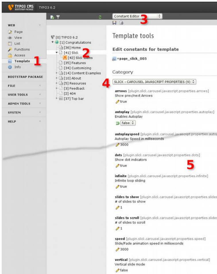
Illustration 35: The TypoScript interface for some Slick properties
